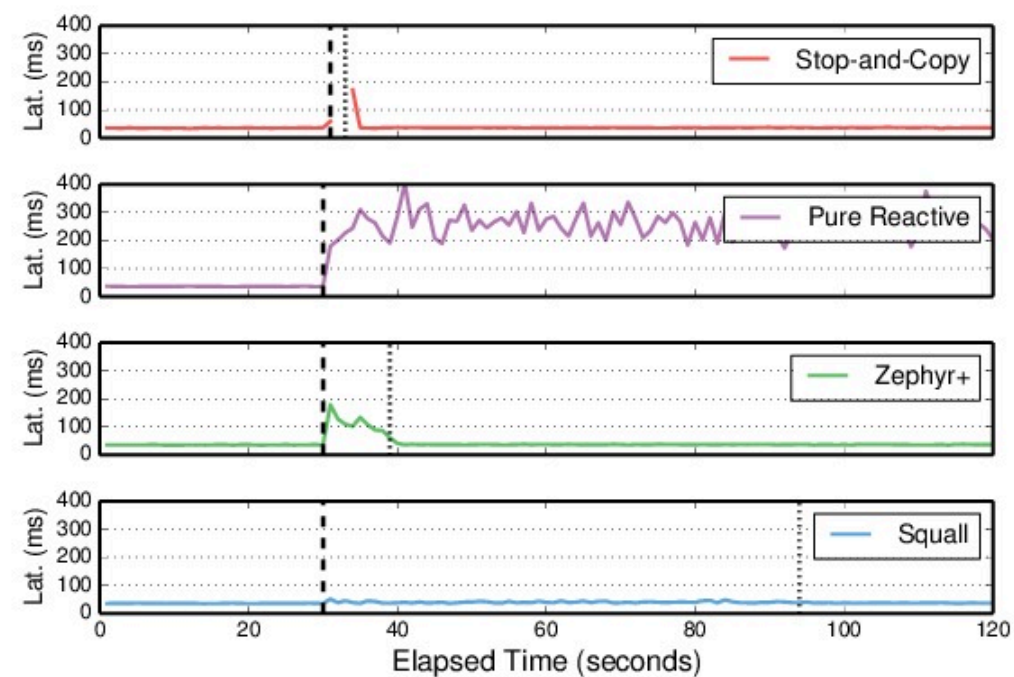
YCSB data shuffle 10% pairwise
